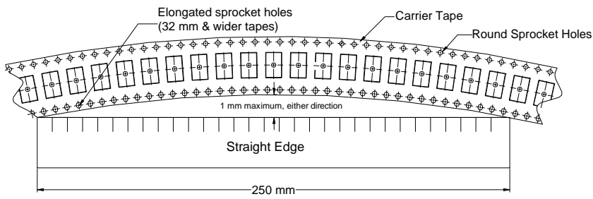
Figure 7 – Maximum Camber
