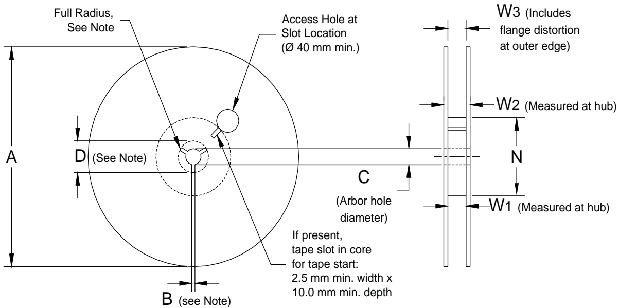
Figure 5 – Reel Dimensions
